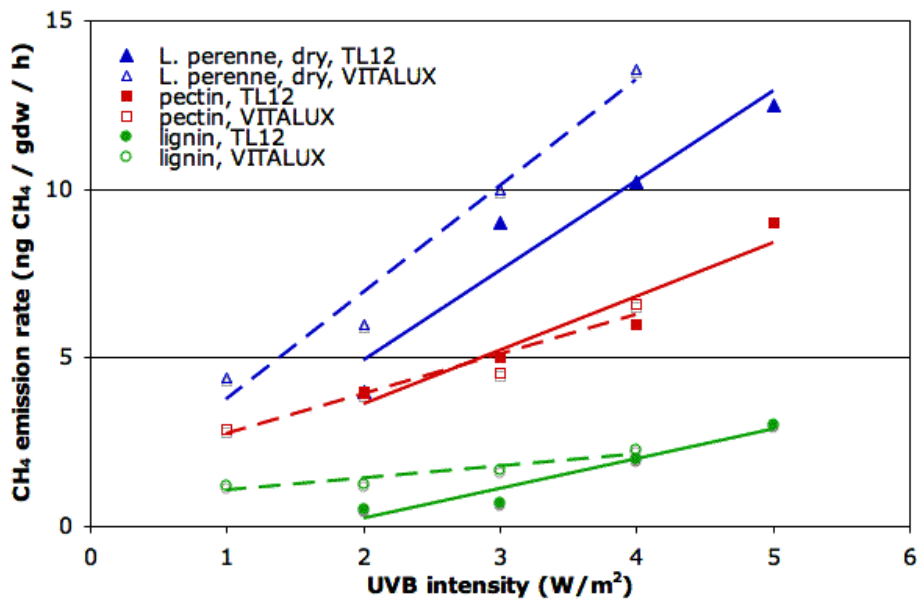
Fig. 2. Dependence of the CH 4 emission rate from dry grass ( L. perenne , blue), pectin (red) and lignin (green) on UVB intensity over the naturally occurring UVB range (unweighted) using the TL12 (solid symbols and linear trend lines) and the VITALUX (open symbols and dashed linear trend lines) lamps.
