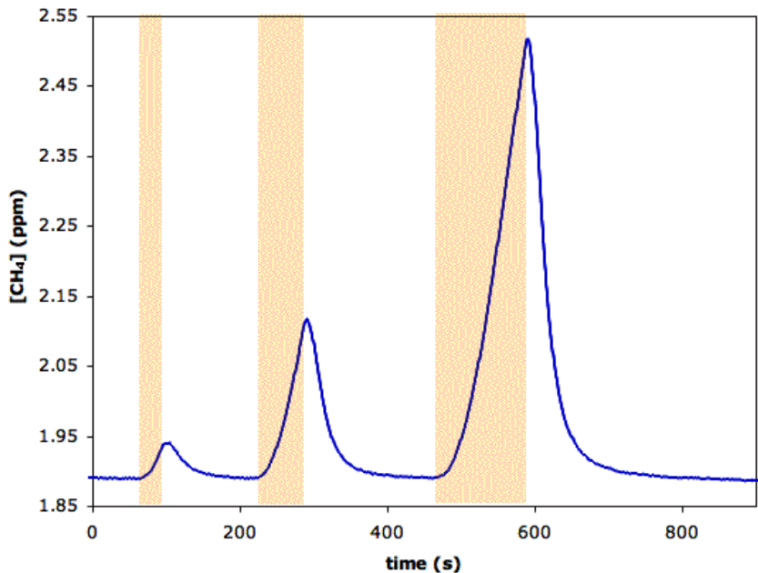
Fig. 7. Response of a grass sample ( Lolium Perenne ) to UV irradiation ( 189\text{ W/m}^2 UVA and 27\text{ W/m}^2 UVB irradiance, Vitalux lamp). The shaded areas mark the times of illumination with the UV light source for 30, 60 and 120 s, corrected for the flushing time of the vial and connecting lines. This flushing time was determined by adding a spike of \text{CH}_4 at the inlet. It is about one minute, in agreement with the size of the vial (100 ml) and the flow rate (100 ml/min). Taking this delay into account the response of the plant matter to light is almost instantaneous.
