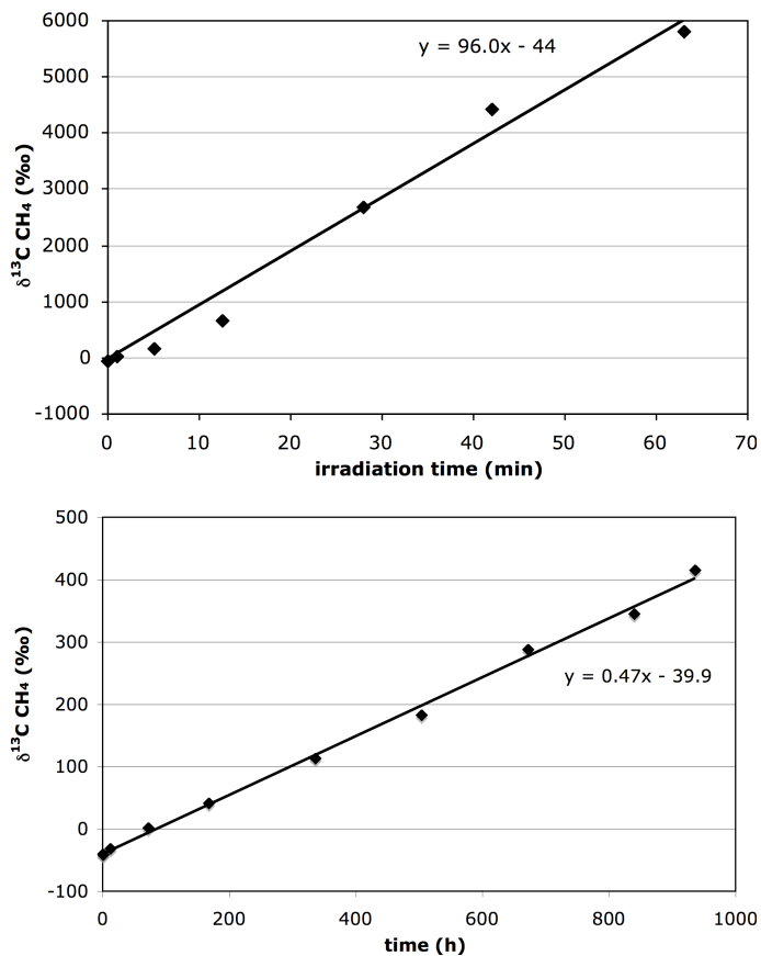
Fig. 8. ^{13}\text{C CH}_4 emission observed from a dry, senesced ^{13}\text{C} labeled wheat leaf ( Triticum aestivum ; 98 atom % ^{13}\text{C} ) under UV irradiation from the VITALUX lamp ( \sim 5 \text{ W/m}^2 UVB) (a) and in the dark without UV (b) in two different static volumes (A, 40 ml; B, 500 ml, see text).
