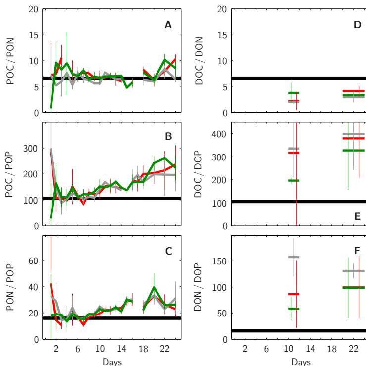
Fig. 10. Temporal development in element ratios of particulate organic and dissolved organic matter produced in the mesocosms' upper surface waters. Ratios shown are POC/PON (A), POC/POP (B), PON/POP (C), DOC/DON (D), DOC/DOP (E), and DON/DOP (F). Ratios of particulate organic matter were determined from organic matter build-up starting from t_0-t_1 averages in each mesocosm (A, B and C). Ratios of dissolved organic matter were estimated from corresponding build-up until the peak and end of the bloom, t_{11}-t_{12} and t_{20}-t_{24} , respectively, starting from t_0-t_4 averages (D, E and F). Style and color-coding follow that of Fig. 5. Black horizontal lines denote respective Redfield ratios.
