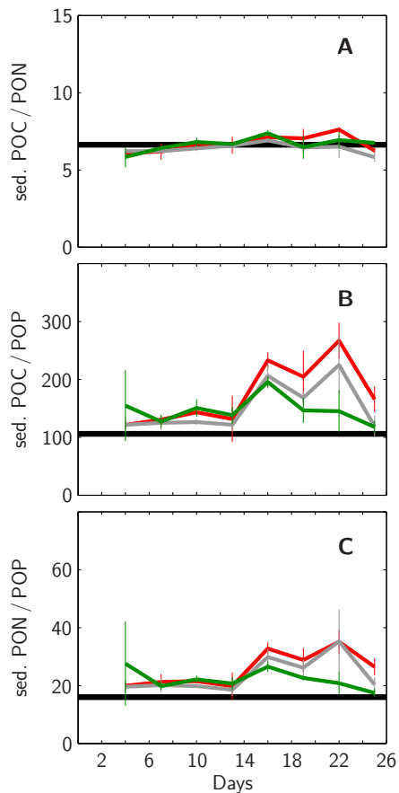
Fig. 11. Temporal development in elemental ratios of particulate organic matter sampled by sediment traps. Shown are sedimentary ratios of POC/PON ( A ), POC/POP ( B ), and PON/POP ( C ). Style and color-coding follow that of Fig. 5. Black horizontal lines denote respective Redfield ratios.
