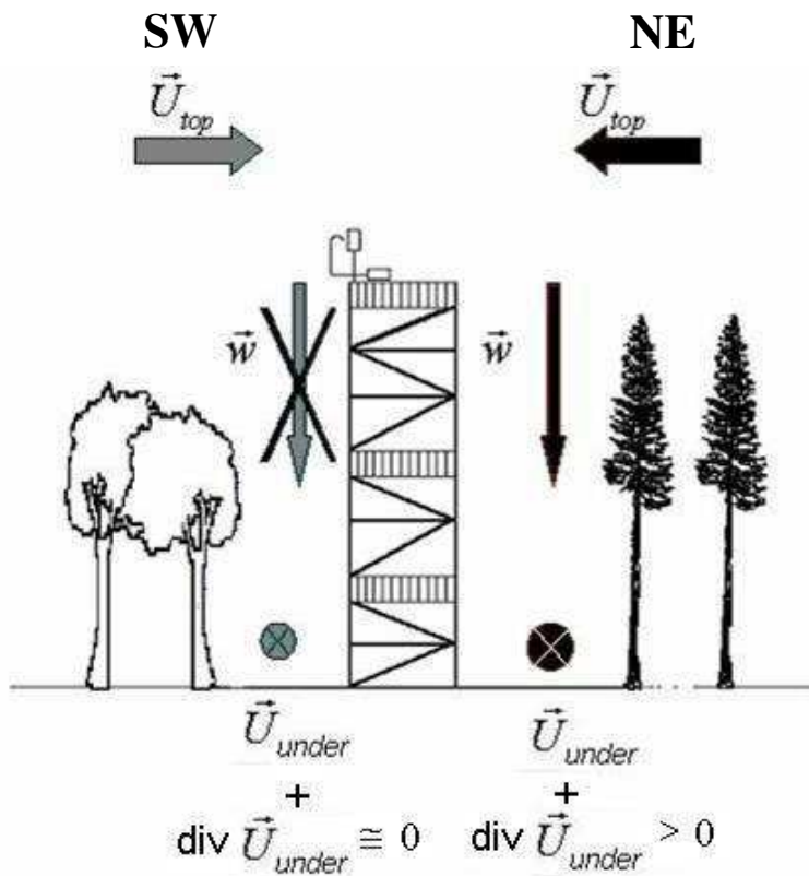
Fig. 8. Schematic representation of the two types of general flow patterns above and in the forest in nocturnal stable conditions. The slope direction is perpendicular to the sheet and inward.
