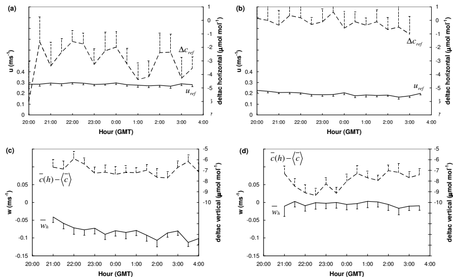
Fig. 9. Mean nocturnal evolution of (a) and (b) the horizontal wind component at the reference level (solid line), the horizontal [CO 2 ] at the reference level (dash line); (c) and (d) the ambient vertical wind component (solid line), the vertical [CO 2 ] difference (dash line). Established for periods with gravitational flows in the trunk space and above-wind direction from the NE sector (a) and (c) or the SW sector (b) and (d). Error bars represent standard error of the mean.
