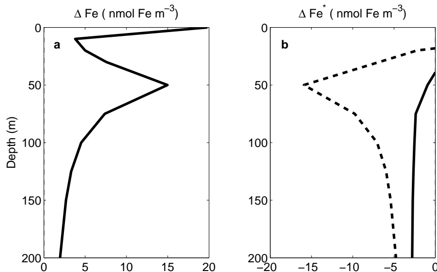
Fig. 12. Vertical profiles of anomalous iron parameters averaged over the eastern tropical Pacific analysis region for the STANDARD case. (a) Anomalous dissolved iron, and (b) \Delta Fe^* (see text for definition) (solid line); \Delta Fe^* if all iron was lost (dashed line). The quantity \Delta Fe^* is a measure of the abundance of anomalous iron and anomalous dissolved inorganic carbon relative to the requirements for phytoplankton. Shown are the results for our 10 year fertilization.
