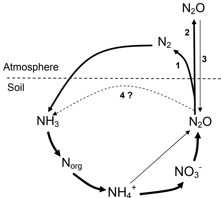
Fig. 1. Origin and possible fate of N 2 O in soil. (1) Complete denitrification to N 2 before escape from the cell; (2) escape from cell; (3) re-entering a cell and subsequent reduction to N 2 , or (4) assimilatory reduction to NH 3 . The ecological relevance of pathway (4) in natural soil is unknown and the focus of this study.
