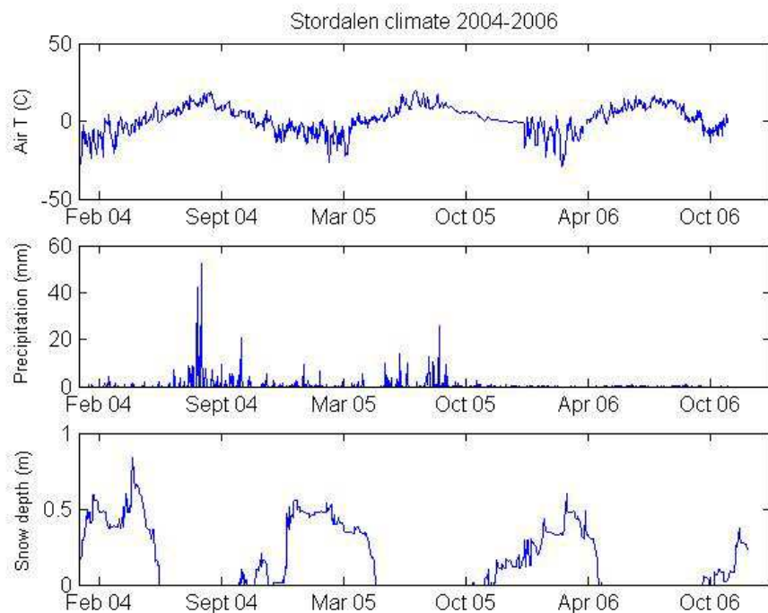
Fig. 3. Three years weather data records from the Stordalen Mire (source: Abisko Scientific Research Station).
