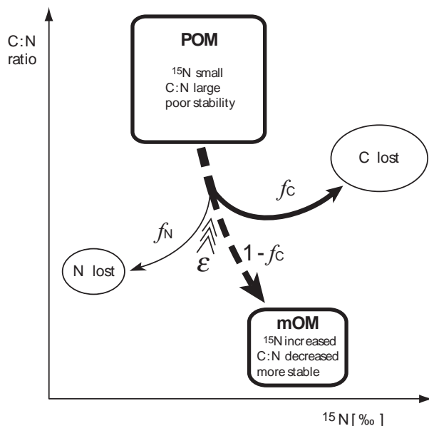
Fig. 1. Conceptual model of the transition of organic matter from particulate organic matter (POM) to mineral-associated organic matter (mOM). Knowledge of the fractionation factor \epsilon and differences in \delta^{15}\text{N} provide information on the fraction of N lost in the process ( f_N ). In addition to changes in C:N ratio, the fraction of lost C ( f_C ) can be calculated. The fraction of C turning into mOM ( 1-f_C ) and the concentrations of POM and mOM provide a measure of the stability of mOM in relation to the stability of POM (Eq. 3 in text).
