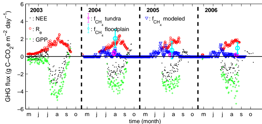
Fig. 12. The seasonal cycles of GPP , R_{\text{eco}} , NEE and f_{\text{CH}_4} . The individual data points represent daily total fluxes, except for the observed methane fluxes (data points with errorbars) which represent weekly averages. The time axis is compressed in the winter months.
