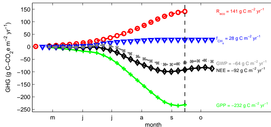
Fig. 14. Annually cumulative GPP , R_{\text{eco}} , NEE and methane fluxes and the resulting GHG balance. The numbers at the right indicate the total flux in mid September, indicated by the vertical dashed line, when eddy covariance measurements were no longer available.
