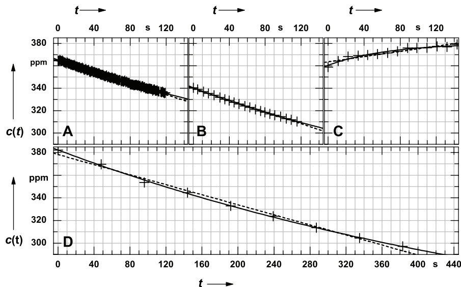
Fig. 2. Examples of the CO 2 concentration c(t) evolution over time t for the different investigation sites. (A) Salmisuo, 11 August 2005, (B) Vaisjeäggi, 17 August 1998, (C) Linnansuo, 12 November 2004, (D) Samoylov, 26 July 2006. The dashed lines indicate linear regression functions f_{\text{lin}} , the solid lines indicate exponential regression functions f_{\text{exp}} . The absolute values of the initial slopes of the exponential functions f'_{\text{exp}}(t_0) are around 0.3 \text{ ppm s}^{-1} for all examples. An overview of the different set-up characteristics is given in Table 1.
