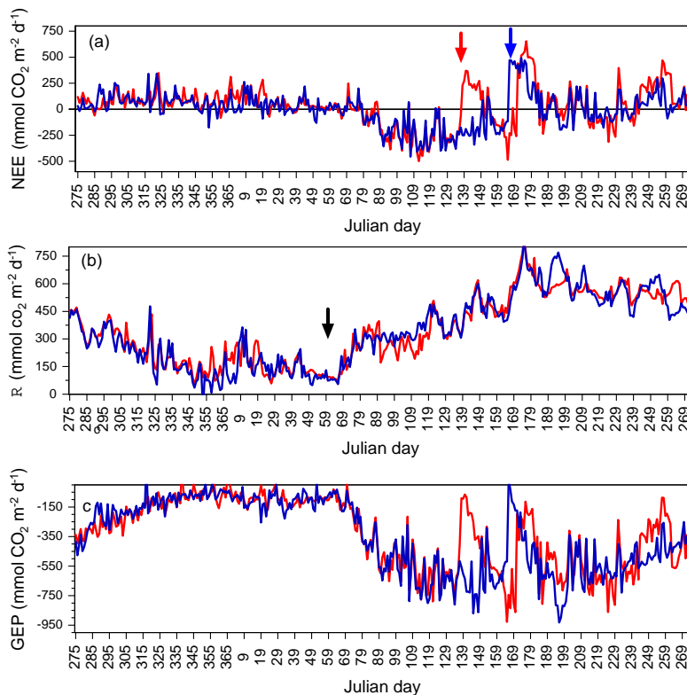
Fig. 10. Seasonal variation in daily values of net ecosystem exchange (a) , ecosystem respiration (b) and gross ecosystem exchange (c) . (Period October 2004 to September 2005; all graphs; Blue line: Stein, extensive management; red line: Oukoop, intensive management). (a) net ecosystem exchange (NEE) (arrows indicate two major grass cutting events in each site.) (b) Ecosystem respiration ( R ) (arrow indicates temperature and respiration increase early March 2005). (c) Gross ecosystem photosynthesis (GEP).
