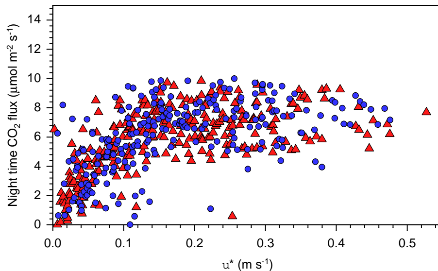
Fig. 6. Relationship between night-time CO 2 flux (half hour averages) and friction velocity ( u^* ) for July 2005, when highest fluxes were observed (blue circles Stein, red triangles Oukoop).
