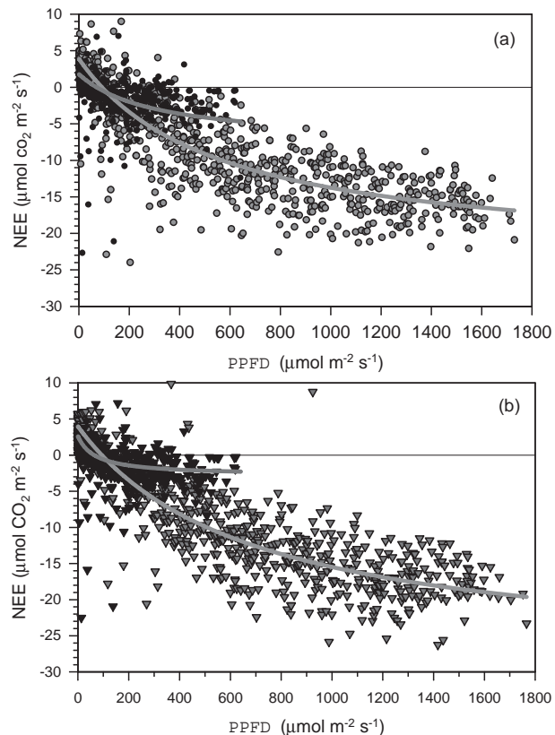
Fig. 7. Relationship between net ecosystem exchange (NEE; half hourly values) and photosynthetic photon flux density (PPFD).
