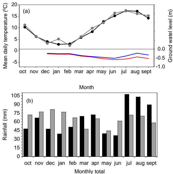
Fig. 2. (a) Monthly (grey circles: Stein) and 30 year average (black circles: period 1975–2005), temperature and ground water level (blue line: Stein; red line: Oukoop; period December 2004–September 2005). (b) Rainfall (black bars: October 2004 to September 2005; grey bars: 30 year average; period 1975 to 2005).
