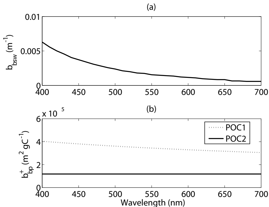
Fig. 4. Modeled (a) backscattering coefficient by sea water b_{bsw} (m -1 ) and (b) carbon-specific backscattering coefficients b_{bp}^+ by small POC (POC1) and large POC (POC2) from 400 nm to 700 nm.
