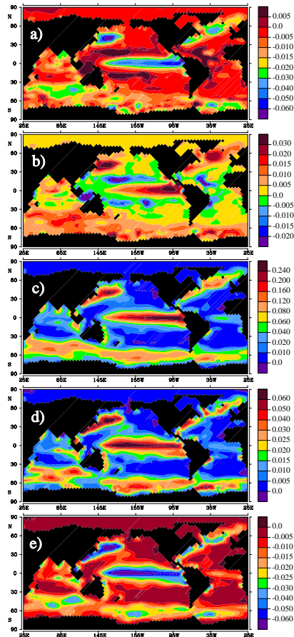
Fig. 6. Regional sensitivity map of air-sea CO 2 flux toward (a) phytoplankton maximum growth rate, (b) phytoplankton exudation, (c) herbivores ingestion, (d) zooplankton grazing, and (e) zooplankton excretion parameters over ten year periods. Negative values indicate that an increase in the correspondent variable will increase the uptake of CO 2 from the atmosphere. Units are in [Pg C].
