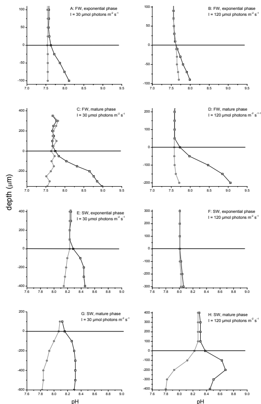
Fig. 6. pH micro profiles measured in biofilms of the exponential (a, b, e and f) and mature phase (c, d, g and h) in a freshwater (FW) at 30°C (a–d) and a marine (SW) biofilm at 25°C (e–g) at 100 l/h flow. The biofilms have been grown at two irradiances: 30 (a, c, e and g) and 120 \mu\text{mol photons m}^{-2} \text{s}^{-1} (b, d, f and h). Open circles represent pH profiles measured in the dark, closed squares represent pH profiles measured in the light.
