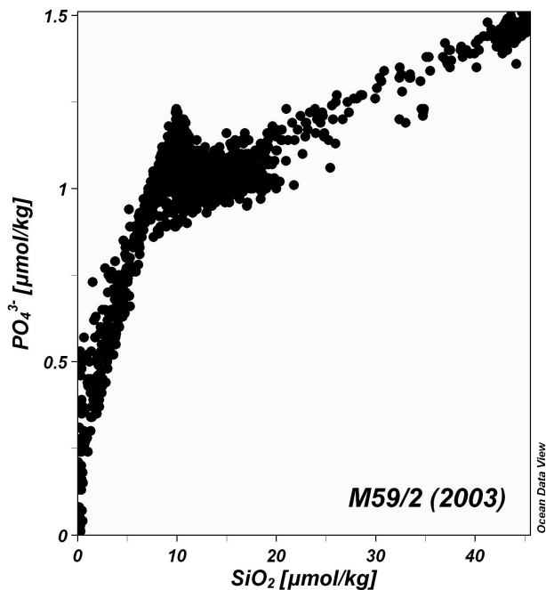
Fig. 5. Phosphate vs. silicate plot of the M59/2 cruise in the entire sNA. The phosphate-silicate relation shows concurrent linear increases of both parameters with depth with a distinct change of the relationship at about 12 \mu\text{mol kg}^{-1} . According to the change the plot is divided into two parts: (I) Silicate concentrations <12 \mu\text{mol kg}^{-1} reflect phosphate and silicate changes from particle remineralization and dissolution in the sNA; (II) silicate concentrations >12 \mu\text{mol kg}^{-1} , concentration changes mainly indicate diapycnal mixing between lower-concentration northern NADW components with higher-concentration AABW.
