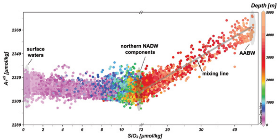
Fig. 6. Salinity adjusted alkalinity by the regional method ( A_T^{eS} ) vs. silicate concentration. Note scale change at 12 \mu\text{mol kg}^{-1} . Colored scale is depth.
