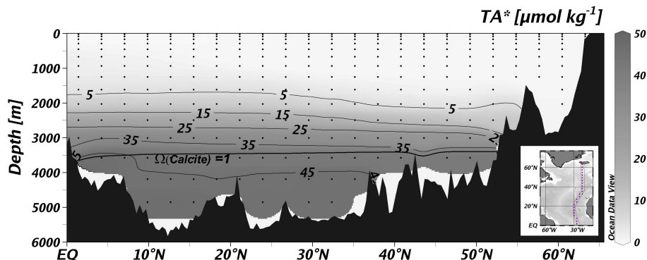
Fig. 7. Model results from the MIT gcm, output as annual mean. Meridional section of excess alkalinity, TA^* , and the saturation horizon of calcite in the North Atlantic along A16. TA^* is defined as alkalinity from dissolution of CaCO_3 below the surface layer and is normalized to the moles of calcium carbonate that have been dissolved.
