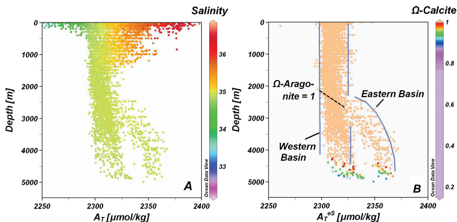
Fig. 3. Hydrographic profiles of alkalinity ( A_T ) from all measurements, color-coded with salinity (A) . (B) Normalized alkalinities ( A_T^{eS} ) using a regional normalization method. The color-coded calcite saturation state ( \Omega ) is calculated from measured alkalinity and total dissolved inorganic carbon (cf. methods). The position of the aragonite saturation horizon is also shown.
