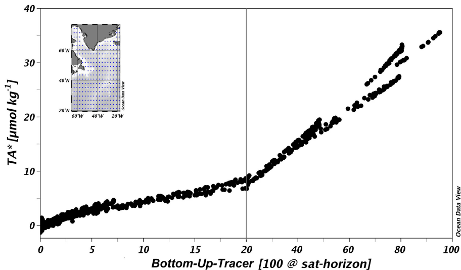
Fig. 8. Model results from the MIT gcm, output as annual mean. Excess alkalinity vs. a diagnostic bottom-up-tracer.
