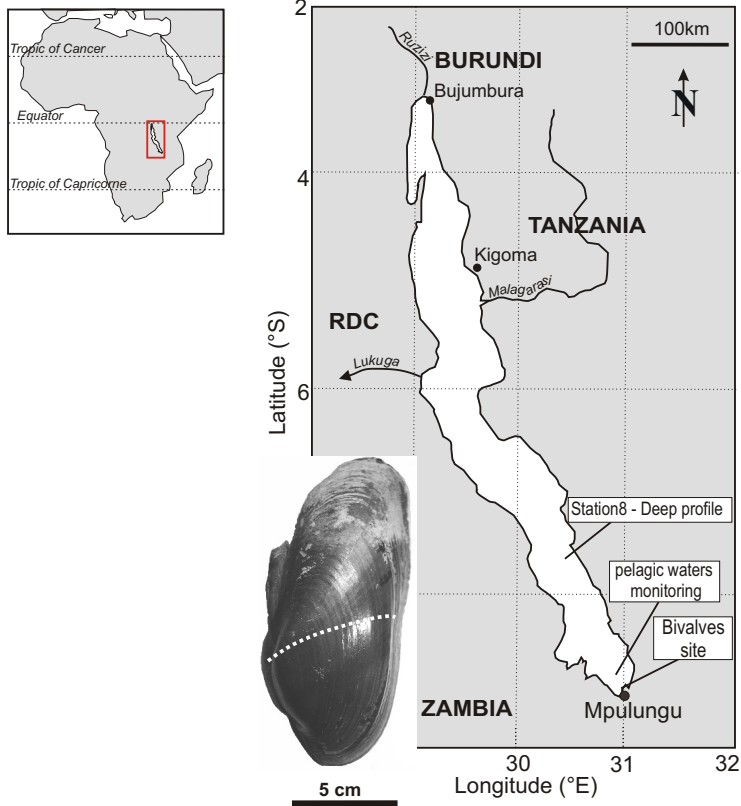
Fig. 1. Location of the study area and sampling sites, in the South of the Lake Tanganyika, where an upwelling occurs seasonally. The lake houses many endemic species such as bivalves Pleiodon spekii (inset). Skeletal Mn profiles were done along radial sections in the anterior part of the shell (white dotted line) because it is preserved from biocorrosion.
