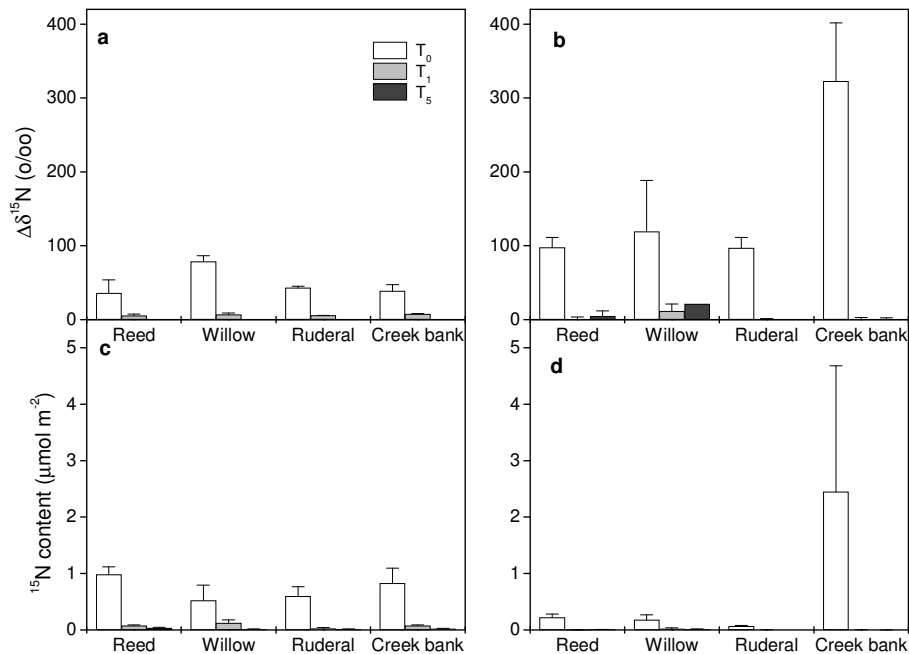
Fig. 6. (a, b) Isotopic enrichment ( \Delta\delta^{15}\text{N} ) and (c, d) amount of ^{15}\text{N} (excess ^{15}\text{N} ) per unit surface area ( \mu\text{mol m}^{-2} ) in material deposited on the sediment surface (filter traps).
