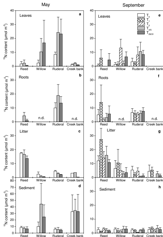
Fig. 4. Amount of ^{15}\text{N} (excess ^{15}\text{N} ) per unit surface area ( \mu\text{mol m}^{-2} ) recovered in the four main compartments ( a, e ) leaves, ( b, f ) roots, ( c, g ) litter and ( d, h ) sediment in the four marsh habitats (reed, willow, ruderal and creek bank) during May and September (Mean \pm SE, n=3 ; n.d.: not determined). T_1 and T_2 was only sampled in September. In May T_5 and T_{31} was sampled, while T_4 and T_{29} was sampled in September. Note the different scale on the y-axis in panels d and h.
