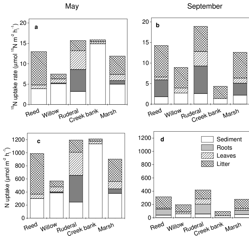
Fig. 8. Total ^{15}\text{N} uptake rate ( \mu\text{mol m}^{-2} \text{h}^{-1} ) ( a, b ) and corresponding absolute N uptake rate ( c, d ) normalized to per hour inundated in May and September. Results are based on \text{T}_0^{15}\text{N} recovery and inundation duration (see text).
