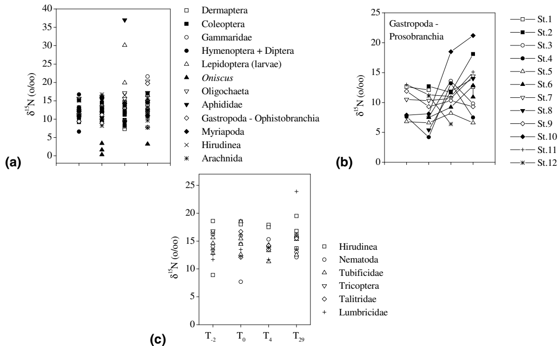
Fig. 7. Isotopic value ( \delta^{15}\text{N} ) in (a) hand-picked invertebrates excluding gastropods (all stations), (b) gastropods collected from the 12 sampling stations, and (c) invertebrate infauna (all stations) on the four sampling occasions in September.
