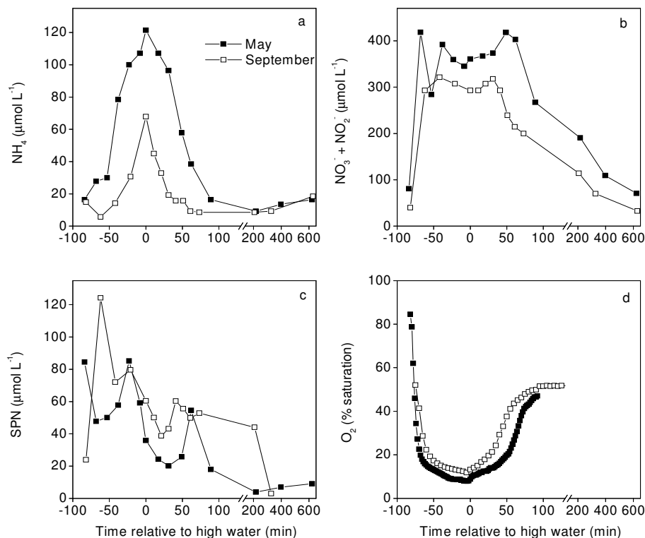
Fig. 2. (a) dissolved ammonium (b), dissolved nitrate + nitrite, (c) suspended particulate nitrogen (SPN), and \text{O}_2 saturation during T_0 (tracer addition) in May and September. Only data from T_0 are shown, as the temporal patterns of all parameters were quite similar among tides on both occasions. (For details see Gribsholt et al., 2005, 2006).
