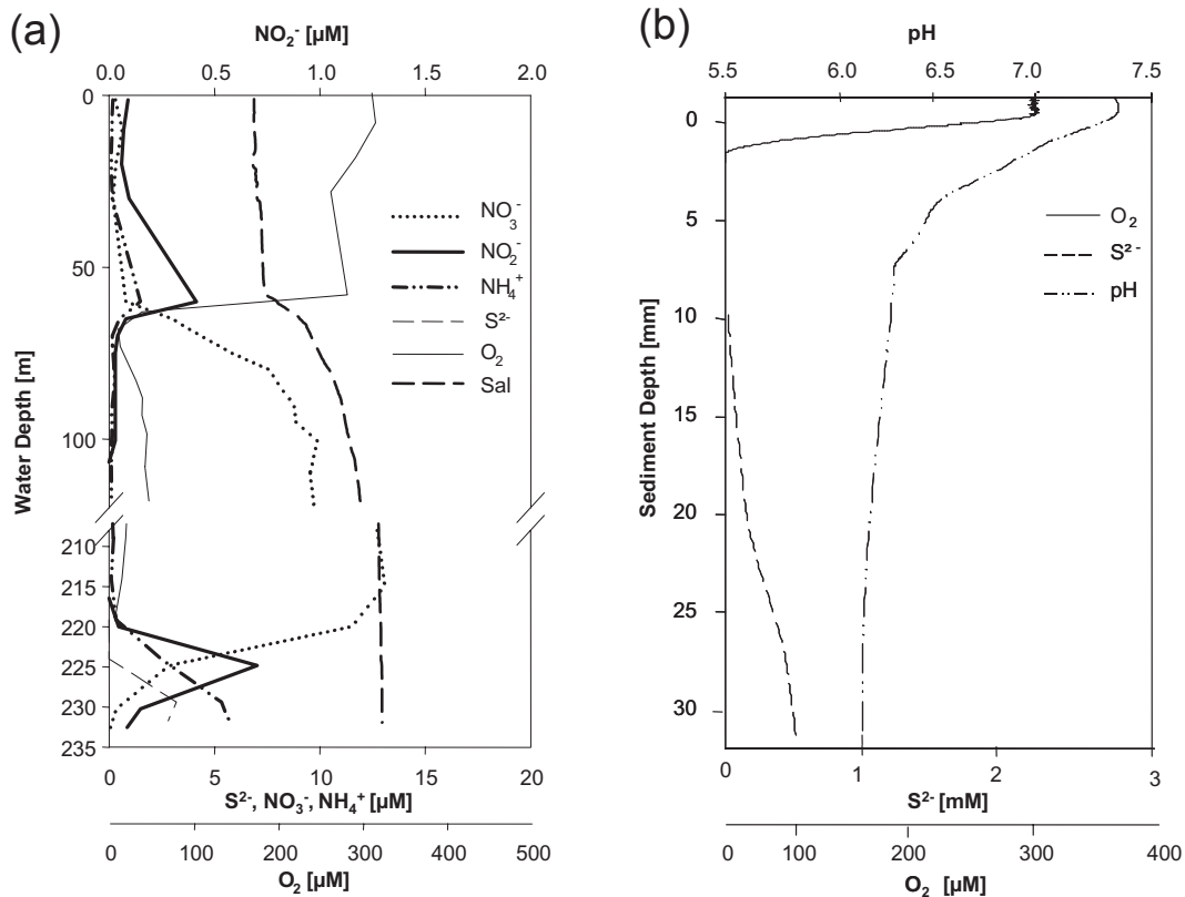
Fig. 2. Physical and chemical parameters of sampling sites in the Baltic Sea; (a) water column in the Gotland Deep, (b) coastal sediment in the Bodden.
