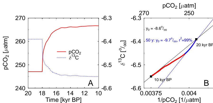
Fig. 10. Effects of iron fertilisation in the Southern Ocean on atmospheric carbon records with scenario taken from Köhler et al. (2005a) (A: p\text{CO}_2 , \delta^{13}\text{C} ; B: Keeling plot). Blue dots and regression in (B) over the first 50 years during p\text{CO}_2 rise only.
