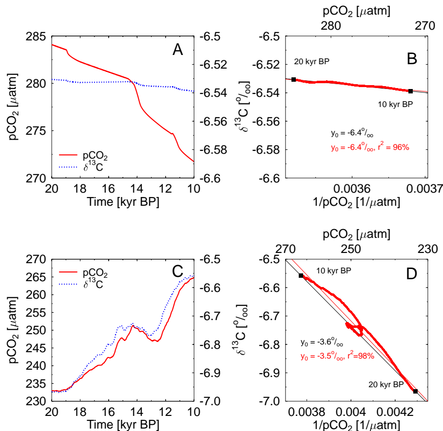
Fig. 13. Simulated effects of sea level rise (top) and ocean temperature change (bottom) as used in Köhler et al. (2005a) (left: \text{pCO}_2 , \delta^{13}\text{C} ; right: Keeling plot). Regression of the prior/after analysis (black) and over the whole period (red) are shown.
