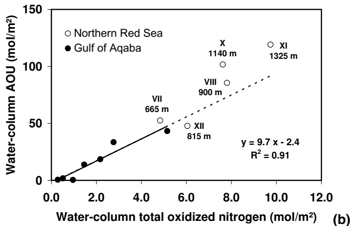
Fig. 6. Apparent oxygen utilization and nutrient remineralization of (a) phosphate, and (b) total oxidized nitrogen follow the “Redfield” stoichiometry in the Gulf of Aqaba and in parts of the northern Red Sea. Note, that for stations IV and V nutrient and oxygen data are not from the same day (see Table 2). Station numbers and maximum sampling depths are indicated (Table 2).
