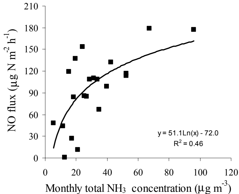
Fig. 4. The relationship between monthly average NO flux and \text{NH}_3 concentrations at the three transect sites downwind of the poultry farm.
