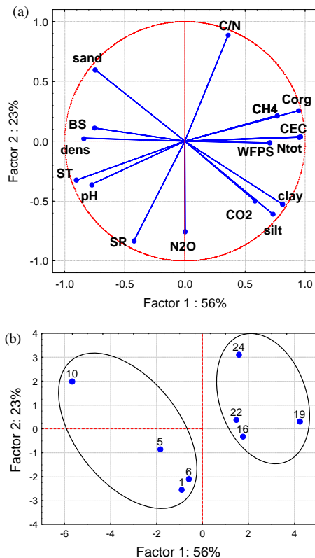
Fig. 5. Loadings plot (a) and scores plot (b) of the PC Analysis. PCA variables: Corg: carbon content; Ntot: nitrogen content; C/N ratio, sand/silt/clay content; BS: base saturation; dens: bulk density; ST: soil surface temperature; pH (water); SR: specific soil respiration; WFPS; water-filled pore space; CEC: cation exchange capacity; N 2 O: N 2 O emissions; CO 2 : CO 2 emissions; CH 4 :CH 4 consumption. PCA cases: NF site (plots 16, 19, 22, 24); PP site (plots 1, 5, 6, 10).
