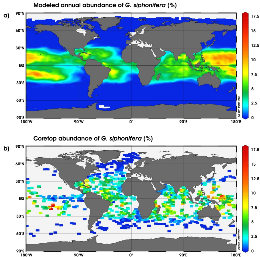
Fig. 8. As in Fig. 5 but for G. siphonifera .
