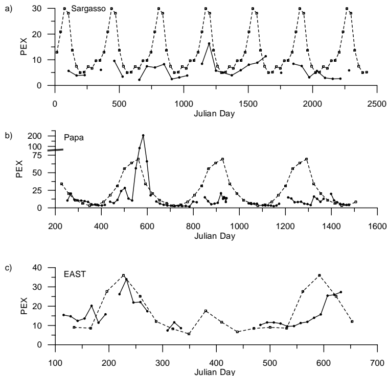
Fig. 13. Comparison of export production values in 1000 m water depth (PEX) calculated for the calibration and the global data set in ( \text{mg C}_{org} \text{ m}^{-2} \text{ d}^{-1} ) for the stations (a) in the Sargasso Sea (Julian Day 1=1 January 1978), (b) at Ocean Station Papa (Julian Day 1=1 January 1982), and (c) in the eastern Arabian Sea (EAST, Julian Day 1=1 January 1986). Solid lines and filled circles show PEX calculated from sediment-trap-derived C_{org} fluxes as applied in the model calibration (for references see Table 1). Dashed lines and open squares show PEX calculated from satellite-derived primary productivity as applied for the global model run after Antia et al. (2001). Trap data are plotted 3 weeks prior to their catchment intervals to account for the time-lag applied in the calibration.
