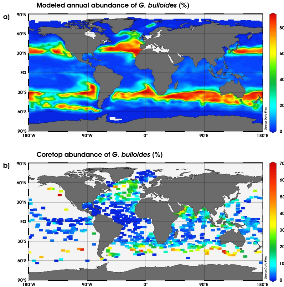
Fig. 7. As in Fig. 5 but for G. bulloides . Note different scaling of color bars.
