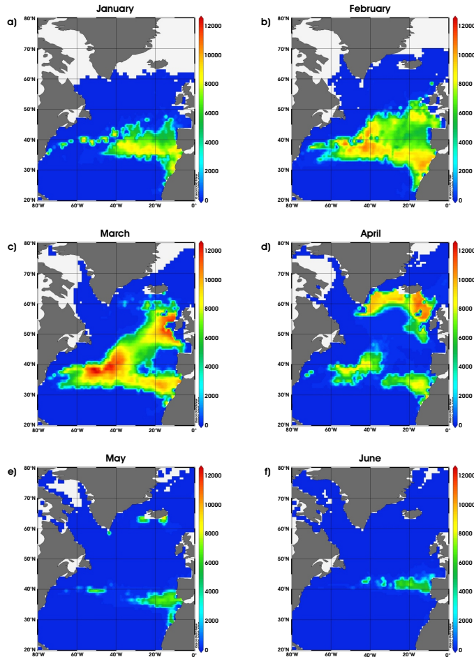
Fig. 14. Modeled monthly fluxes (ind. m -2 d -1 ) of the species G. bulloides in the N-Atlantic for the months January to June (a)–(f).
