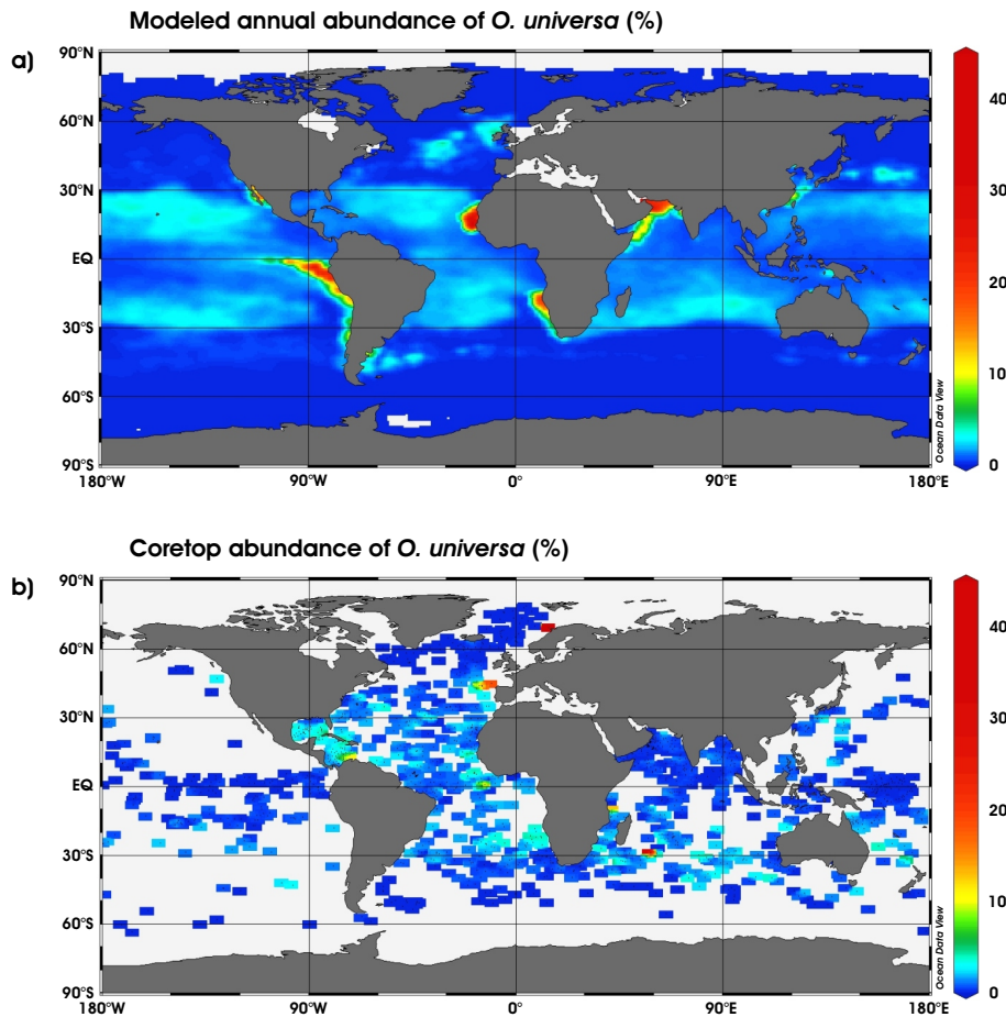
Fig. 10. As in Fig. 5 but for O. universa .
