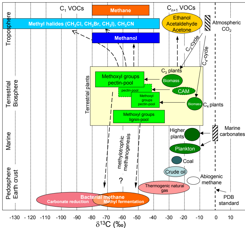
Fig. 2. Schematic diagram displaying 13 C depletion of methoxyl groups relative to bulk biomass of terrestrial plants and their relationship to biospheric C 1 and C n+1 VOCs. Data for carbon isotopic composition of major carbon pools were taken from Whiticar (1996). Carbon isotope signatures for VOCs are related to sources, degradation steps after formation are not taken into account.
