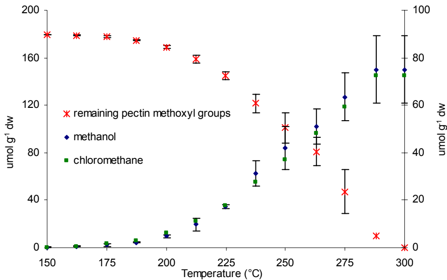
Fig. 1. (c) Remaining pectin methoxyl pool (PM) after each heating step in relation to the formation of methanol and chloromethane.
