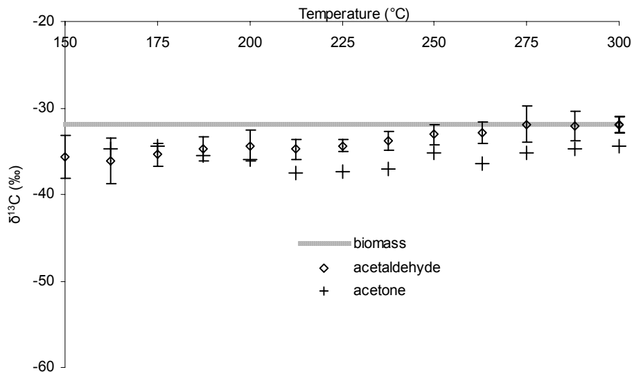
Fig. 1. (d) Carbon isotope composition of accumulated acetaldehyde and acetone at various temperatures during progressive heating of ash leaf biomass with reference to the \delta^{13}\text{C} value of the original bulk biomass. Error bars shown for acetaldehyde are also typical of those for acetone.
