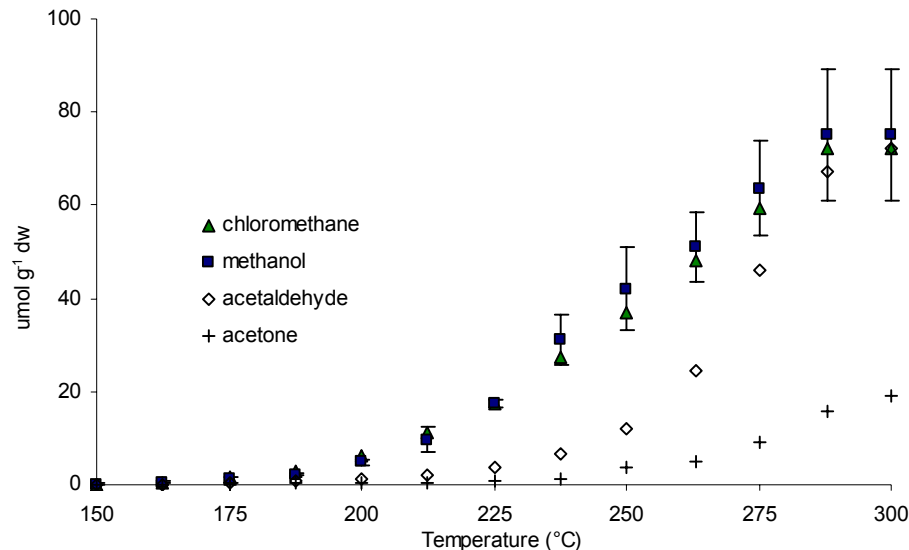
Fig. 1. Amounts and isotopic signatures of several volatile organic compounds formed during progressive heating of lyophilised ash leaves. (a) Cumulative amounts of methanol, chloromethane, acetaldehyde and acetone formed are shown on a molar basis. Each point is the mean of three replicate analyses of independent samples ( n=3 ). Error bars shown for \text{CH}_3\text{OH} are typical of SDs for all compounds.
