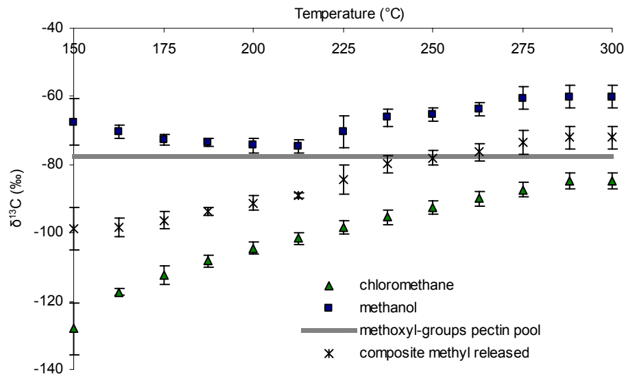
Fig. 1. (b) Carbon isotopic composition of accumulated CH 3 OH and CH 3 Cl at each temperature during progressive heating. Also shown is the composite \delta^{13}\text{C} values calculated on a molar basis for CH 3 OH and CH 3 Cl released during heating. For reference the measured initial \delta^{13}\text{C} of the pectin methoxyl pool is displayed. Vertical bars show SD for triplicate samples.
