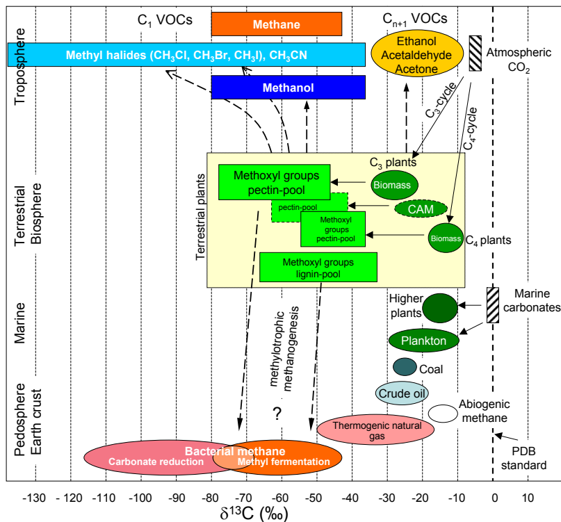
Fig. 2. Schematic diagram displaying ^{13}\text{C} depletion of methoxyl groups relative to bulk biomass of terrestrial plants and their relationship to biospheric \text{C}_1 and \text{C}_{n+1} VOCs. Data for carbon isotopic composition of major carbon pools were taken from Whiticar (1996). Carbon isotope signatures for VOCs are related to sources, degradation steps after formation are not taken into account.
