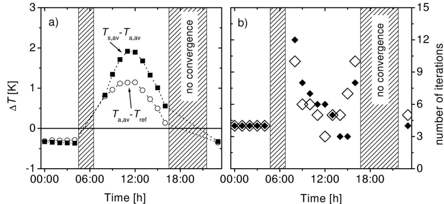
Fig. 2. (a) Diel cycle of the temperature differences between the foliage and the ambient air ( T_{s,av} - T_{a,av} , solid squares) and between the ambient air and the surface layer ( T_{a,av} - T_{ref} , circles), calculated for EUST-I (Fig. 1a, c, f). (b) Number of iterations required to achieve model convergence for EUST-I (closed diamonds) and EUST-II (open diamonds). Simulations for unsteady environmental conditions during sun rise (5–7 h) and sunset (17–22 h) failed to converge as indicated by the hatched areas.
