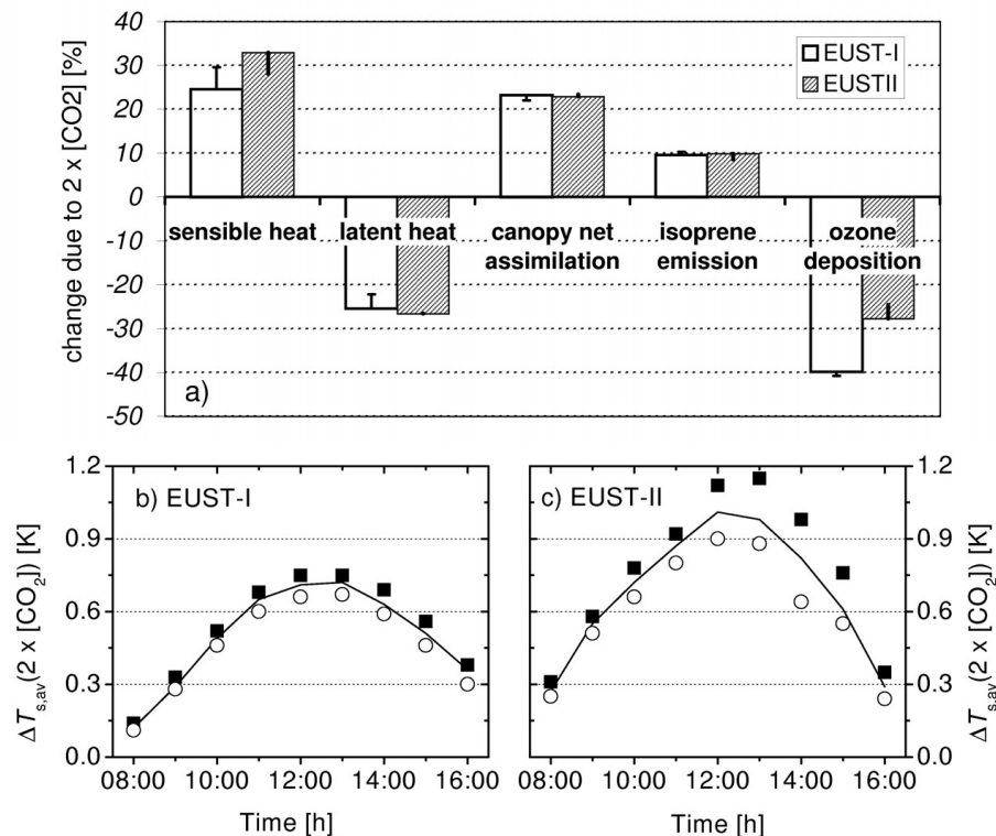
Fig. 13. Calculated impact of doubled atmospheric CO 2 concentrations on canopy fluxes and surface temperatures. (a) Predicted change of energy net fluxes, canopy net assimilation, isoprene emissions and ozone deposition for EUST-I (open bars) and EUST-II (shaded bars). Error bars represent predictions using higher stomatal conductance (EUST-I) and lower photosynthesis (EUST-II) parameters, respectively (see Table 2 in Sect. 2.3). (b, c) Diel course of calculated change in mean surface temperature ( \Delta T_{s,av}[2 \times \text{CO}_2] ) applying the reference parameterization (solid line), higher stomatal conductances (closed squares) and lower photosynthesis parameters (open circles).
