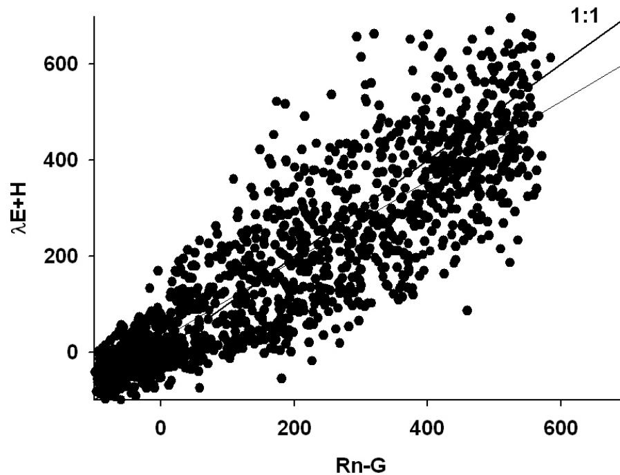
Fig. 1. Energy balance closure test for 30 min averages of the sum of latent and sensible heat versus net radiation minus soil heat flux. The slope of the line is 0.83 with an intercept of 26 \text{ Wm}^{-2} and a r^2=0.79 .
