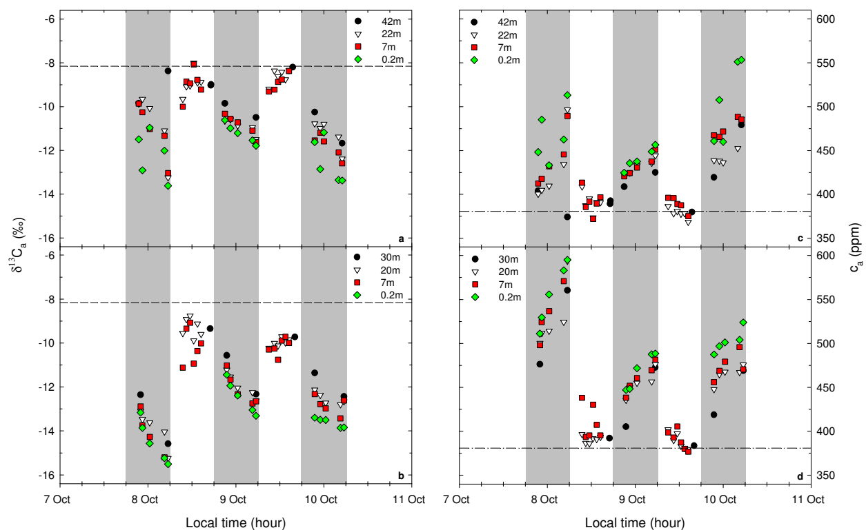
Fig. 5. Diurnal curves of \delta^{13}\text{C}_a and c_a along a topographical gradient in Central Amazonia on 7–10 October 2006: on the plateau ( a , c ) and in the valley ( b , d ). Points correspond to the single measurements made at each sampling level. The dashed line ( a , b ) and the dash-dotted line ( c , d ) represent the carbon isotope ratio of tropospheric background CO 2 ( \delta^{13}\text{C}_b ) and the tropospheric background [CO 2 ] ( c_b ) measured in the marine boundary layer at Ascension Island, UK (7.92° S 14.42° W; 54 m a.s.l.), respectively, on October 2006 (about −8.156‰ and 380.77 ppm). The \delta^{13}\text{C}_b was determined by linear interpolation using the data from October 2004 and 2005, as these were the last data available (about −8.105 and −8.152‰ respectively). The c_b was determined by adding the annual [CO 2 ] growth rate for the year 2006 (about 1.73 ppm year −1 ) to the [CO 2 ] on October 2005 (about 379.04 ppm) (White and Vaughn, 2007; Conway et al., 2007). The shaded boxes indicate the nighttime periods.
