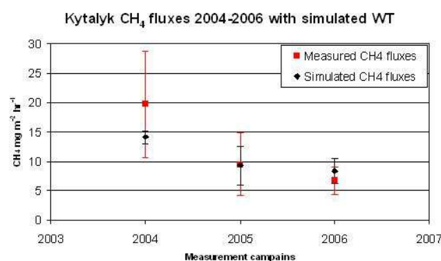
Fig. 11. Average measured value (red) and simulated (black) CH 4 emissions for 2004–2006 at Kytalyk site using the floodplain simulated water table from Fig. 6.
