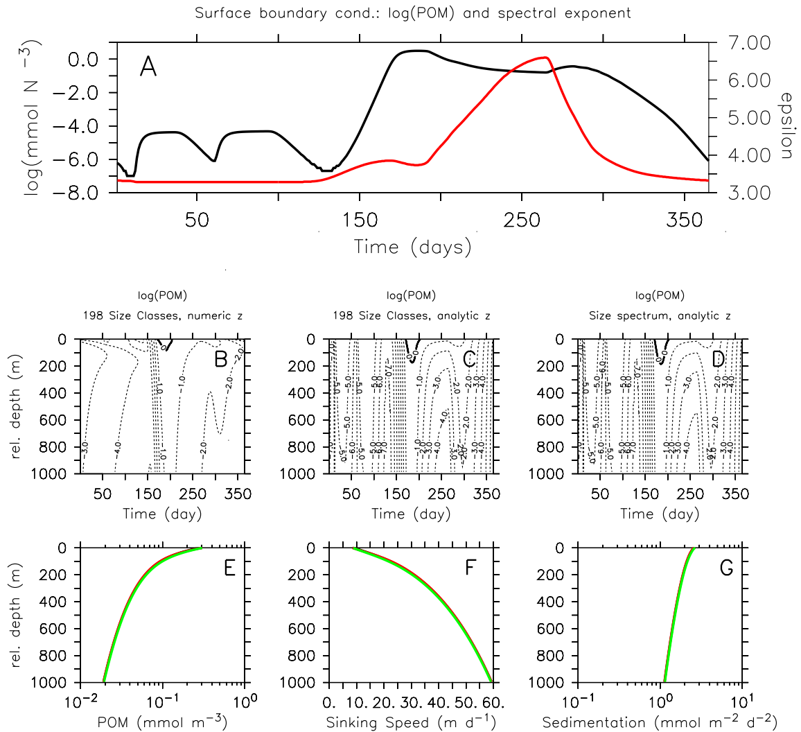
Fig. 8. Results of spectral models with arbitrary seasonal forcing. Panel A: surface boundary conditions, black line – \log(\text{POM} [\text{concN}]) , red line – spectral exponent \epsilon . Panels B–D: \log(\text{POM} [\text{mmol N m}^{-3}]) vs. time and depth, B–198 size classes, numerical integration over depth, C–198 size classes, analytic integration over depth, D – analytic integration over size and depth. Panels E–G: annual averages of POM ( [\text{mmol N m}^{-3}] , E), average POM sinking speed ( [\text{m d}^{-1}] , F) and sedimentation ( [\text{mmol N m}^{-2} \text{d}^{-1}] , G). Lines in panels E–G: black – 198 size classes, numerical integration over depth, red – 198 size classes, analytic integration over depth, green – analytic integration over size and depth. The black and red lines are mostly overlaid by the green line.
