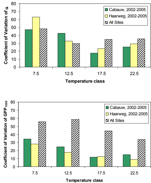
Fig. 5. Coefficient of variation per temperature class of \alpha , (upper frame) and GPP_{1000} (lower frame). The temperature class is indicated by the middle temperature of the class. The CV from interannual variability (Haarweg and Cabauw, 2002–2005) is compared to CV from the intersite variability (year 2005).
