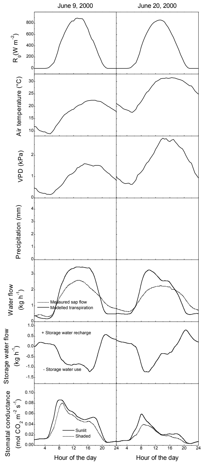
Fig. 8. Comparison of diurnal patterns during two days (9 June and 20 June 2000): climate, water flow and modeled stomatal conductance ( g_s , given per square meter of sunlit or shaded leaf at the top of the canopy) of pine #23. ( R_g = incoming solar radiation; VPD = vapour pressure deficit)
