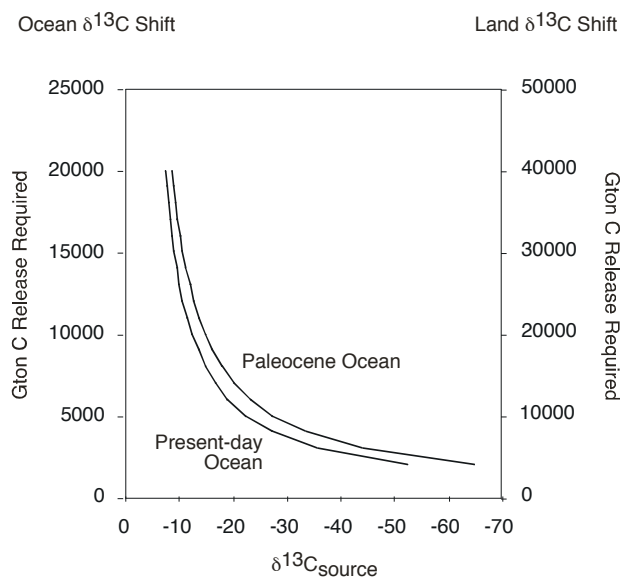
Fig. 8. Size of the implied PETM carbon release as a function of its carbon isotopic composition. The right-hand axis assumes the \delta^{13}\text{C} spike of -2.5\text{‰} as observed in most ocean \delta^{13}\text{C} records. The left-hand axis assumes a global \delta^{13}\text{C} shift from the paleosol records, about twice that in the ocean (Koch et al., 1992). The mass-balance calculation requires an estimate of the ocean inventory of carbon; we show results assuming the present-day ocean carbon chemistry, and that for a Paleocene ocean assuming equilibrium with 600 ppm atmospheric \text{CO}_2 and with solid \text{CaCO}_3 .
