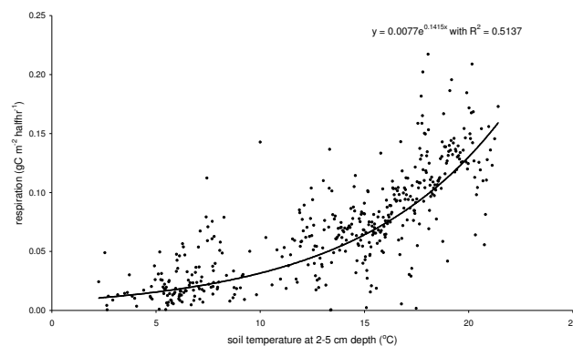
Fig. 6. Relation between soil temperature and respiration using nocturnal CO_2 fluxes with the exponential best fit line and its regression equation.
