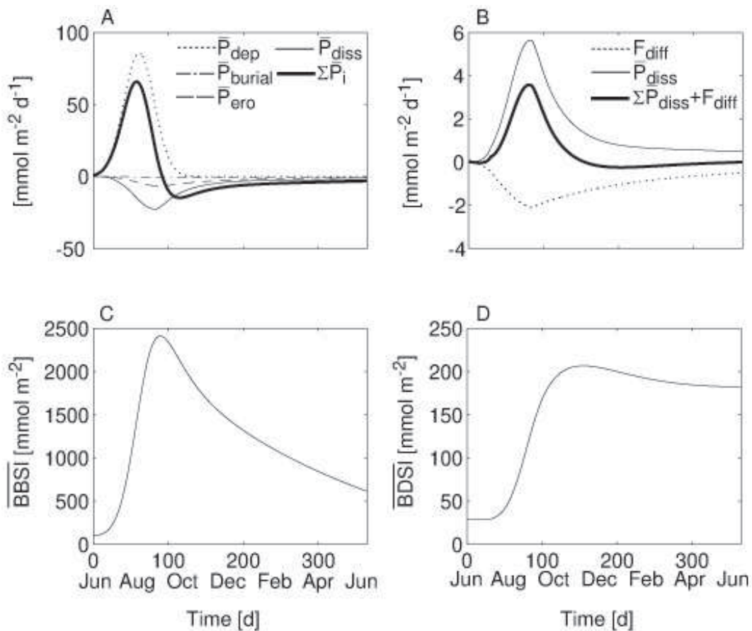
Fig. 3. Temporal evolution of depth-integrated (A) deposition flux \overline{P_{\text{dep}}} , erosion flux \overline{P_{\text{ero}}} , burial flux \overline{P_{\text{burial}}} , dissolution rate of biogenic silica \overline{P_{\text{diss}}} and net rate \Sigma_i \overline{P_i} , (B) depth-integrated dissolution rate \overline{P_{\text{diss}}} , diffusive flux \overline{F_{\text{diff}}} , and net rate \Sigma \overline{P_{\text{diss}}} - \overline{F_{\text{diff}}} (C) depth-integrated biogenic silica content in the sediments BBSI and (D) depth-integrated dissolved silica concentration BDSI. Simulation results correspond to the baseline parameter set (Table 2)
