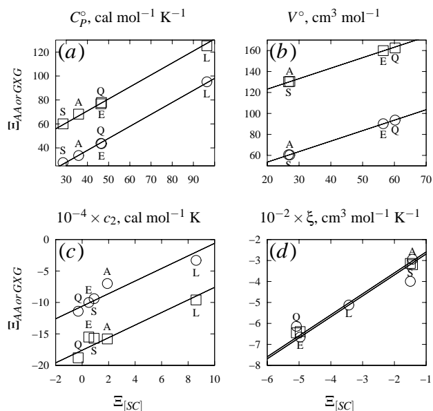
Fig. 7. C_p^{\circ} , V^{\circ} , c_2 , and \xi of model amino acids (□) and Gly-X-Gly tripeptides (○) as a function of the corresponding property of the model sidechain groups. The values of \Xi_{[\text{SC}]} were calculated using Eq. (27) and the group contributions given in Table 6. The values of \Xi_{\text{AA}} and \Xi_{\text{GXG}} were taken from Table 2. The regression lines have slopes of unity and intercepts that correspond to \Xi_{[\text{AABB}]} or \Xi_{[\text{GXGBB}]} .
