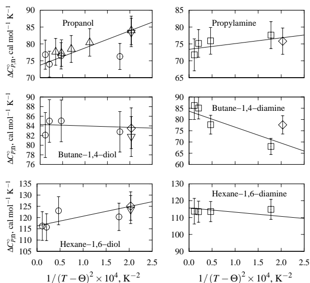
Fig. 6. \Delta C_{p,n}^{\circ} as a function of 1/(T-\Theta)^2 of aqueous propanol, butane-1,4-diol, hexane-1,6-diol, propylamine, butane-1,4-diamine, and hexane-1,6-diamine. Experimental values of C_p^{\circ} were taken from Ingles and Wood, 1996 (○), Ingles et al., 1997 (□), Makhatazde and Privalov, 1989 (△), Jolicoeur and Lacroix, 1976 (▽), Nichols et al., 1976 (◇; alcohols), and Cabani et al., 1981 (◇; amines). The error bars represent an estimated experimental uncertainty of \pm 5\% . The values of c_1 and c_2 , which correspond to the intercepts and slopes of the regression lines, were calculated using the equations given in Table 7 together with the organic group contributions given in Table 6.
