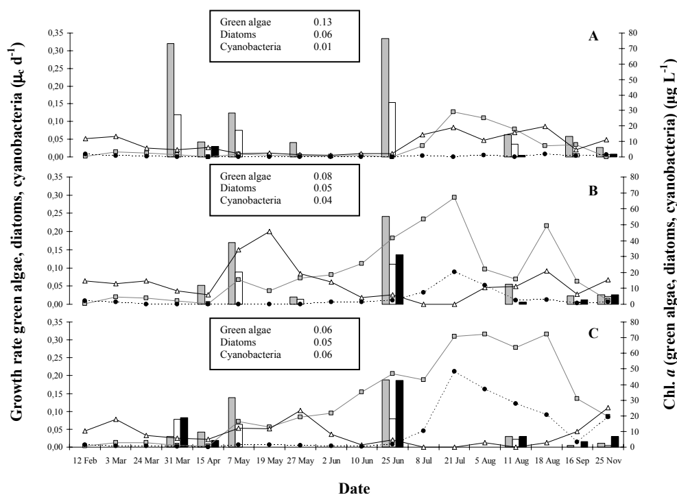
Fig. 4. Growth rates ( \mu_C \text{ d}^{-1} ) and abundances of green algae, diatoms and cyanobacteria ( \mu\text{g Chl. } a \text{ L}^{-1} ). Mean growth rates \sim 18 and \sim 24 h. after incubation are calculated as the ^{13}\text{C} incorporation into the \text{C}_{18:n} FA of green algae (grey column) and cyanobacteria (black column) and \text{C}_{20:5} FA of diatoms (white column). Abundances of the green algae, diatoms and cyanobacteria are given by; the grey line with squares, black line with triangles and dotted line with circles, respectively. Boxes represent the average seasonal growth rate ( \mu_C \text{ d}^{-1} ), per algal group, per treatment.
