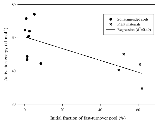
Fig. 2. The relationship between the activation energy and the initial fraction of the fast-turnover pool for the data referred to by Knorr et al. (2005a). A two-pool model, similar to Eqs. (1–2), was fitted to observed data but the activation energy was assumed to be the same for both pools (Kätterer et al., 1998).
