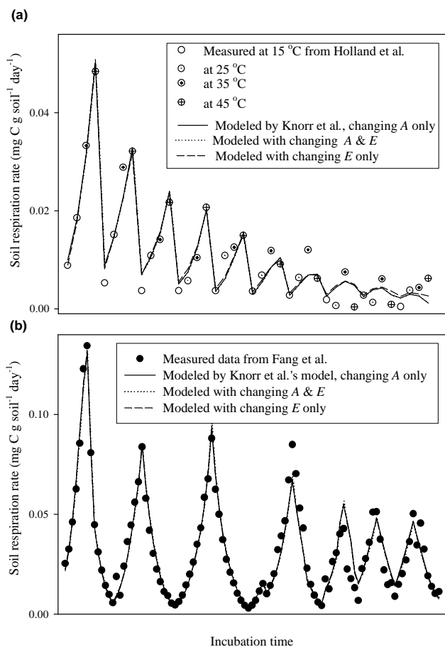
Fig. 1. Comparison between modelled and measured data among models. Measured data are average of all samples. (a) Data from Holland et al. (2000) cited by Knorr et al. (2005a). Soil samples were taken from a tropical forest in Brazil, and were incubated for 24 weeks under different constant temperatures (15, 25, 35, and 45 °C). Sample size was 10–15 g. (b) Measured respiration rate from Fang et al. (2005) for soils under a middle-aged plantation of Sitka spruce in Scotland. Soil samples (4 samples with 4 replicates, each weighed 600–800 g) were incubated for 102 days under changing temperature (4–44 °C, with a step of 4 °C).
