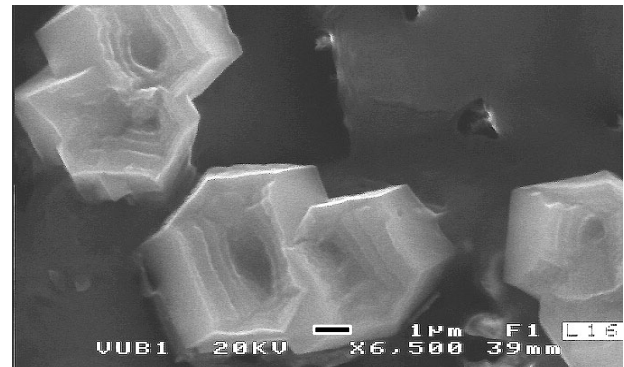
Fig. 16. SEM image of Prismatic bipyramidal Ca-oxalates (weddelite) crystals showing a multi-layer and concentric zonation structures reflecting crystal growth mechanism around a nucleus. Most crystals show a four layer zonation. The crystals nucleated on fungal spores. The size and shape of the nuclei are identical to fungal spores in the growth environment. Black bar scale= 1\text{ }\mu\text{m} .
