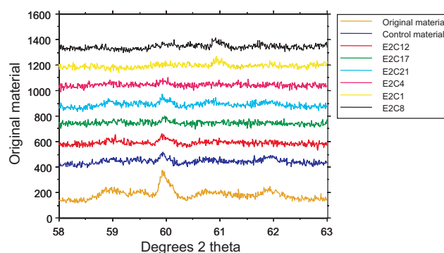
Fig. 9. New mineral peaks in the faecal samples at 60.9^\circ 2\theta in the earthworm-slate experiment.
