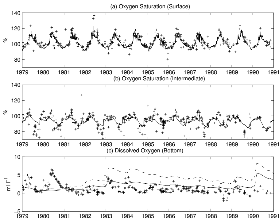
Fig. 6. Observed and simulated oxygen saturation at the surface (a) and in the intermediate layer (b). Panel (c) shows the evolution of the dissolved concentration for the simulation with a relaxation time scale for salinity RTS=90 d (continuous line) and RTS=720 d (dashed line). Negative values are indicative of the presence of HS^- ions.
