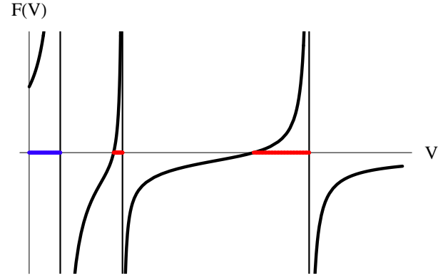
Fig. 1. Generic graph for the existence domains in a three-component plasma. The red ranges yield acceptable necessary conditions, the blue one not. The precise labeling of the asymptotes depends on the ordering of the different thermal velocities.
