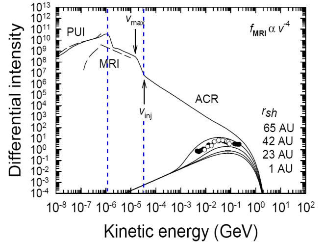
Fig. 9. Differential intensity in particles/(m 2 s sr MeV) of suprathermal particles pick-up ions, PUI; multiply reflected ions, MRI together with that of ACRs. The symbols are Voyager observations of modulated ACR spectra (le Roux et al., 2000). The vertical dashed lines indicate the ion energy range that will become accessible via the plasma instrument of IHP.
