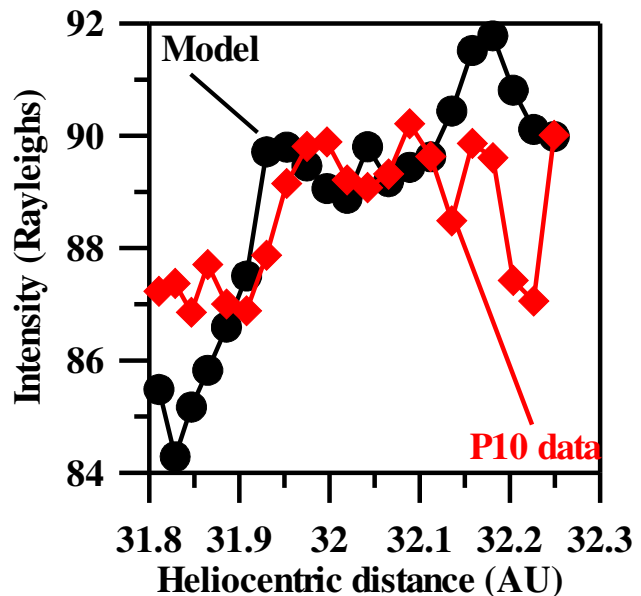
Fig. 1. The calculated intensity for the heliospheric model with neutral hydrogen density of 0.15 cm -3 and proton density of 0.05 cm -3 and P10 intensity modified by a calibration factor of 2.36 are plotted against spacecraft heliocentric distance. The standard error for the calculated intensity in this and subsequent figures is calculated by the equation given in the text.
