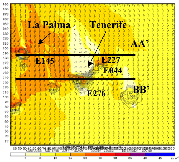
12:00 UTC 28 November 2005
