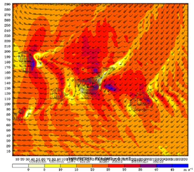
00:00 UTC 29 November 2005
