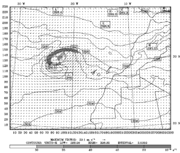
12:00 UTC 28 November 2005
