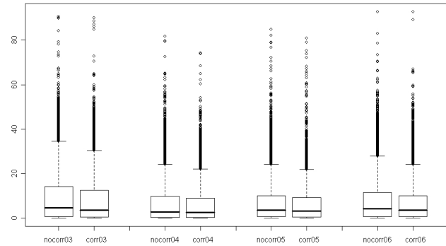
Figure 4. Comparison of annual boxplots of the uncorrected and corrected FWI series in the period 2003–2006.
