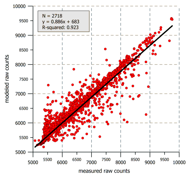
Figure 4. Scatterplot of ANN-modeled and measured hourly cumulative raw counts of LWS 3 at Christnach; data from 2.4.2007 to 24.7.2007.
