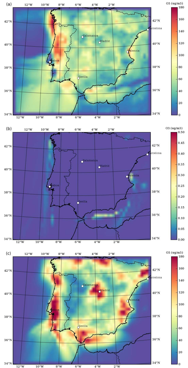
Figure 3. Factor separation analysis. Hourly maximum impact. (a) S'_A , pure contribution of anthropogenic emissions to ozone formation; (b) S'_B , pure biogenic contribution; (c) S'_{AB} , mutual interaction between anthropogenic and biogenic emissions.
