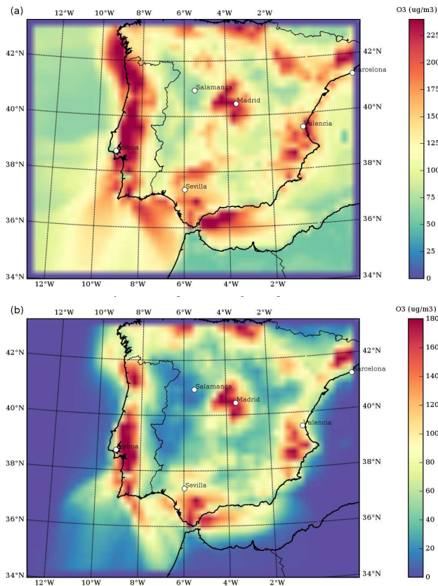
Figure 2. (a) Hourly maximum of ozone for every grid during the episode. (b) Maximum hourly impact of biogenic emissions, S_{AB}-S_A ( \mu\text{g}/\text{m}^3 ) for the 10–15 August 2003 episode. Note that the difference does not necessarily occur on the ozone peak.
