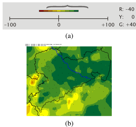
Figure 6. As in Fig. 5 but showing the effect of a zero-centered, yet compressed colour range.
