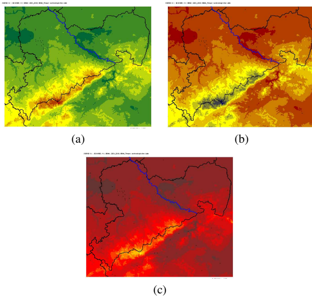
Figure 2. Three views of the same state. Shown is the annual mean temperature distribution in Saxonia applying different colour schemes. (a) Green/yellow/red; (b) blue/yellow/red and (c) yellow/red. The colours in each subfigure are assigned so that they cover a value range from +3 to +10^{\circ}\text{C} .
