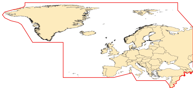
Figure 2. The WMO RA VI Region.
