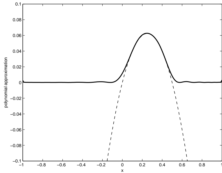
FIGURE 3. Positive polynomial approximation of degree 50 (solid) of the positive piecewise-polynomial function \max(0, g_1) on [-1, 1] . Polynomial g_1 is represented in dashed line.
