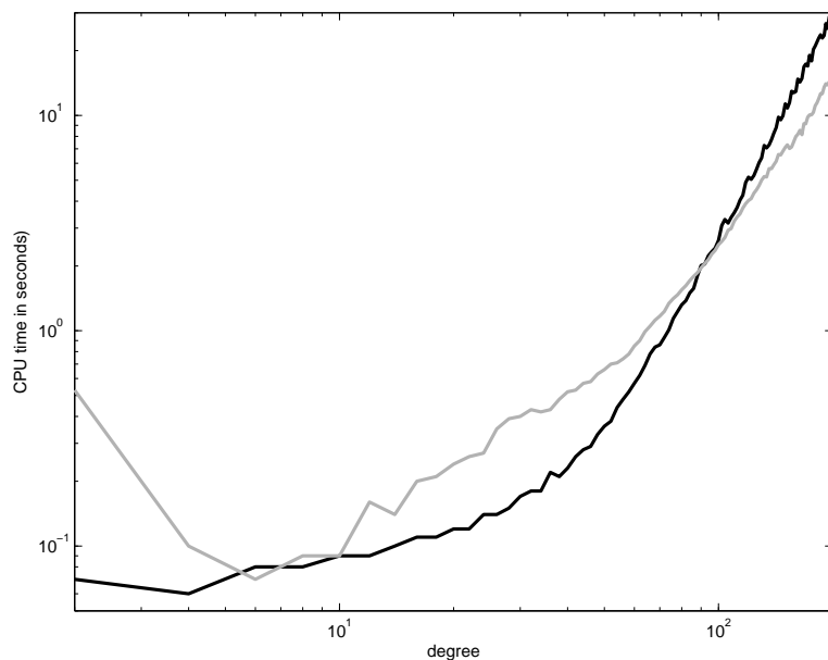
FIGURE 8. CPU time required to solve the SDP relaxations (Chebyshev basis in black, power basis in gray) as a function of the degree.
