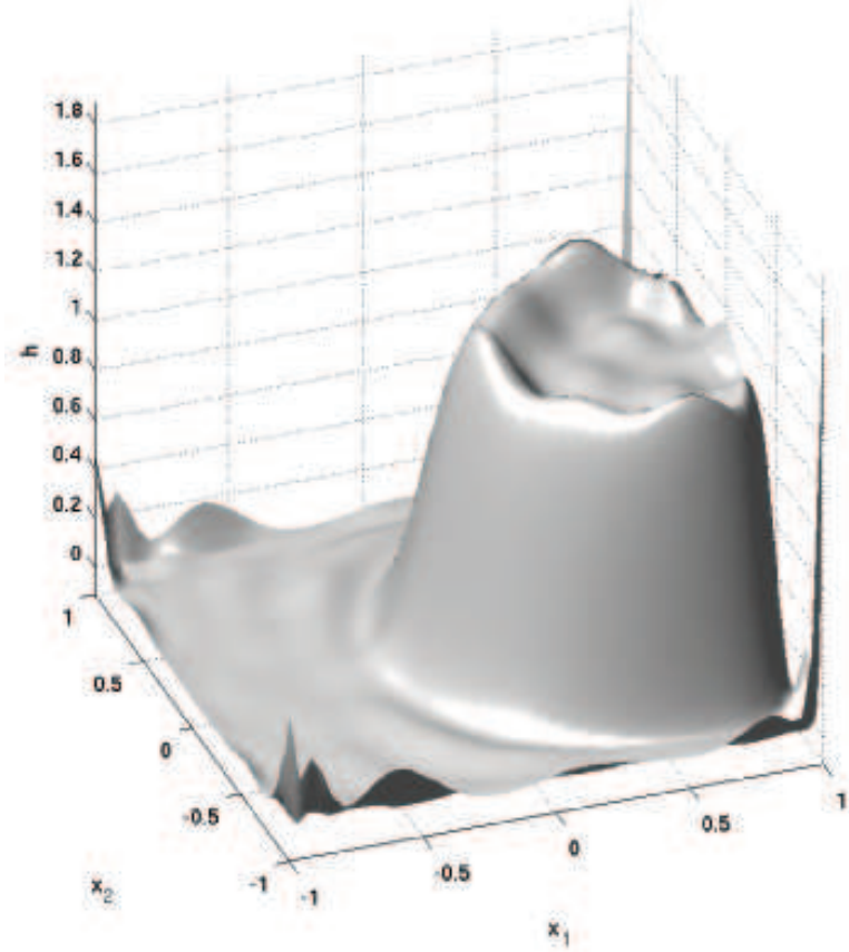
FIGURE 10. Positive polynomial approximation of degree 20 of the indicator function of the bean surface.
