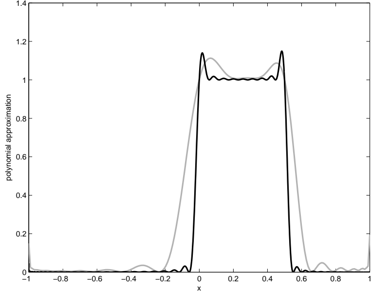
FIGURE 6. Positive polynomial approximation of degree 100 of the indicator function I_{[0, \frac{1}{2}]} in the Chebyshev basis (black) and power basis (gray).
