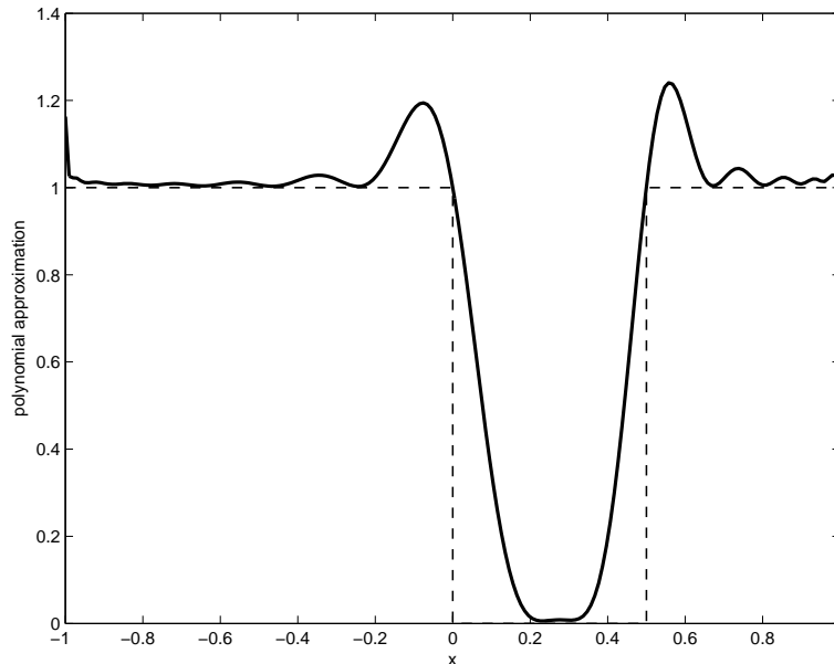
FIGURE 4. Positive polynomial approximation of degree 50 (solid) of the complementary indicator function 1 - I_{[0, \frac{1}{2}]} (dashed) on [-1, 1] .
