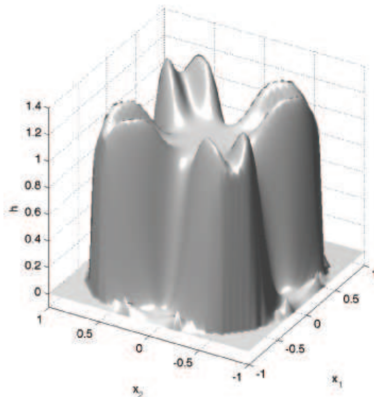
FIGURE 13. Positive polynomial approximation of degree 20 of the indicator function of the folium surface.
