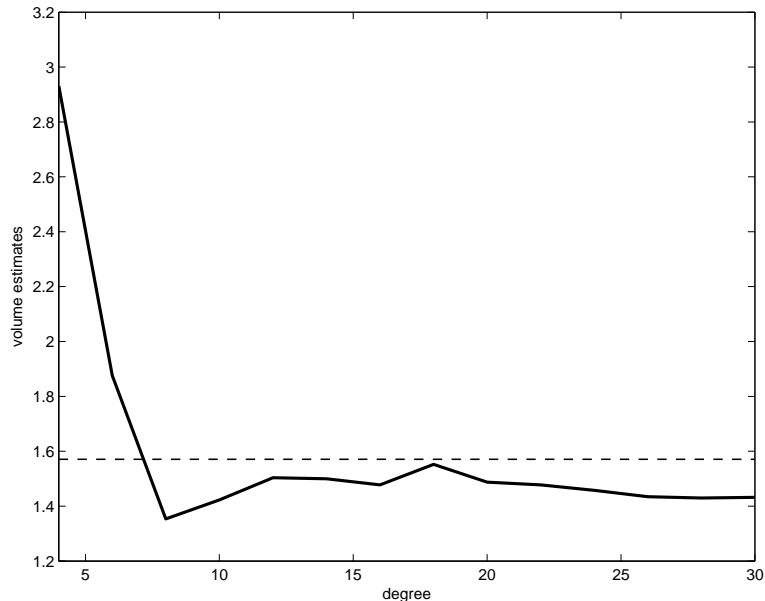
FIGURE 12. Approximations of the area of the folium obtained by solving SDP relaxations of increasing degree.
