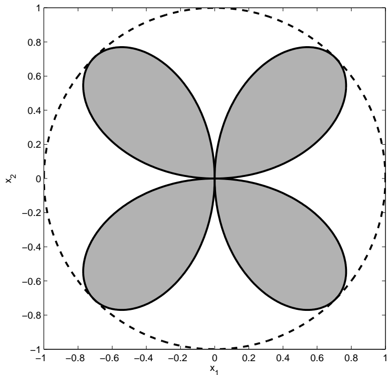
FIGURE 11. Folium surface.
