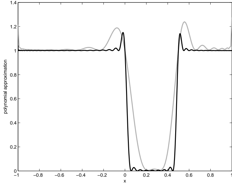
FIGURE 7. Positive polynomial approximation of degree 100 of the indicator function 1 - I_{[0, \frac{1}{2}]} in the Chebyshev basis (black) and power basis (gray).
