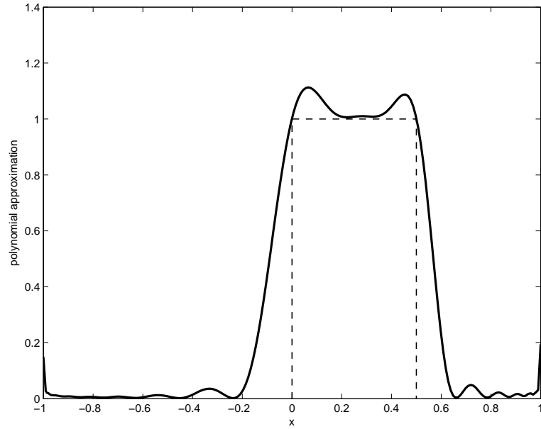
FIGURE 2. Positive polynomial approximation of degree 50 (solid) of the indicator function I_{[0, \frac{1}{2}]} (dashed) on [-1, 1] .
