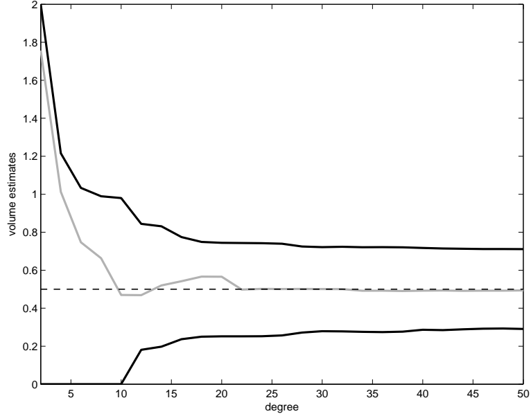
FIGURE 1. Three sequences of approximations of \text{vol}[0, \frac{1}{2}] obtained by solving SDP relaxations of increasing degree.
