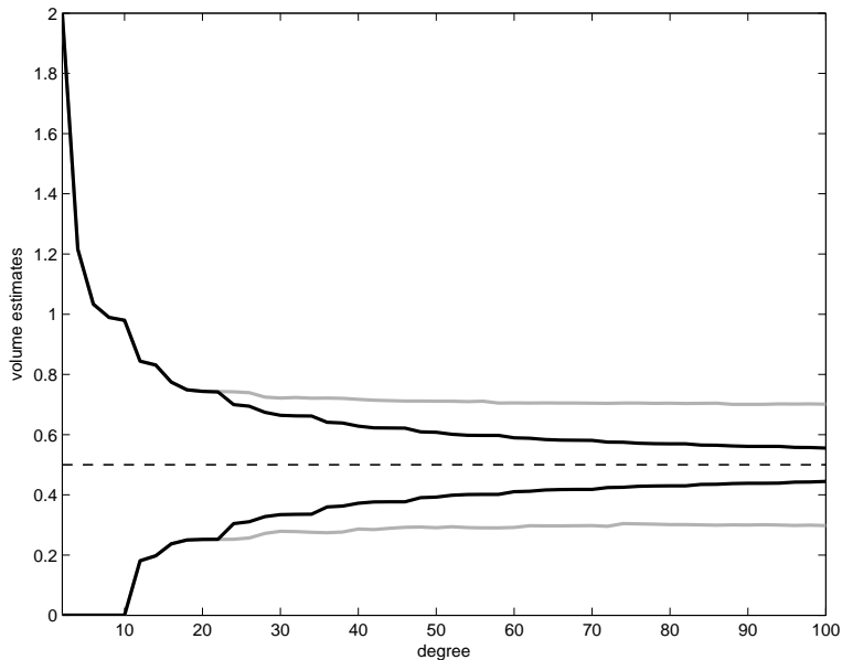
FIGURE 5. Upper and lower bounds on \text{vol}[0, \frac{1}{2}] obtained by solving SDP relaxations in the Chebyshev basis (black) and power basis (gray).
