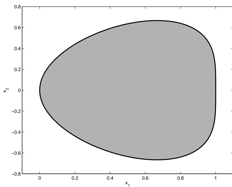
FIGURE 9. Bean surface.
